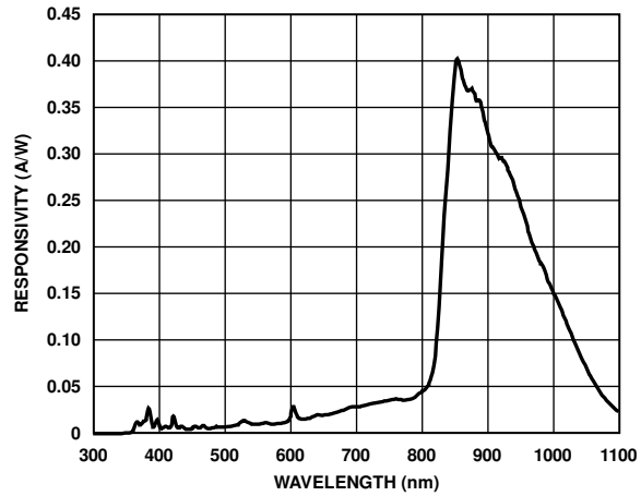
Figure 7. Responsivity vs. Wavelength (Angle = 0°)
