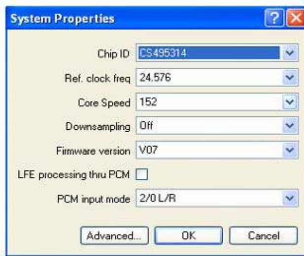
Figure 4-2. System Properties Showing CS495314 as the Chip ID
