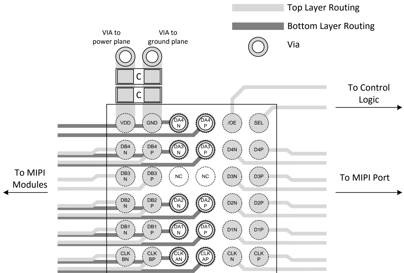
Figure 31. Layout Example
