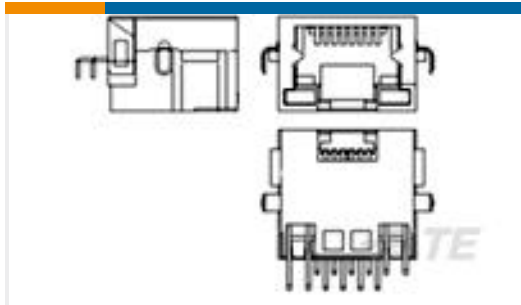
TE Part #1-1775399-7 MOD JACK, RJ45, GRAY, REEL, 30u" AU
