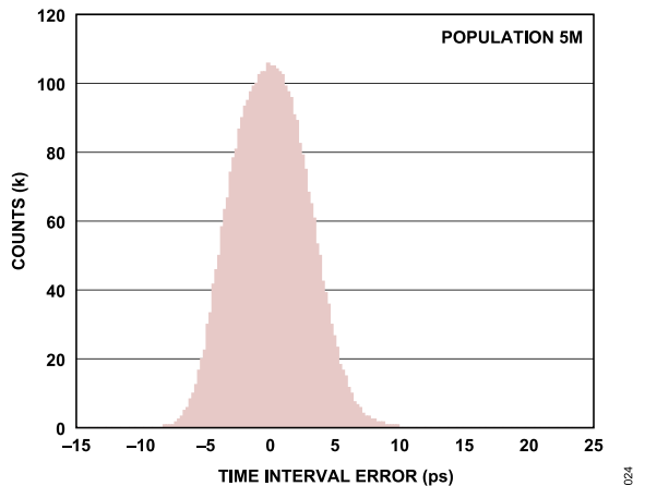
Figure 32. Time Interval Error (TIE) Histogram for D_{OUT\pm} at 1.25 GHz
