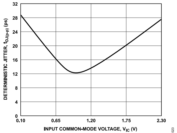
Figure 31. Deterministic Jitter, t_{DJ(p-p)} vs. Input Common-Mode Voltage, V_{IC}
