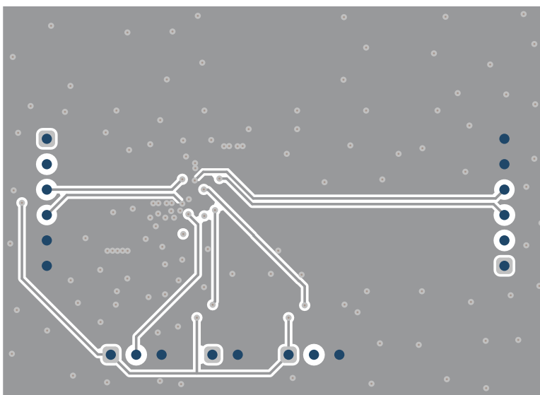
Figure 5-4. Signal Layer 2
