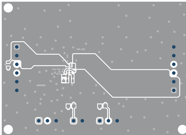
Figure 5-2. Top Layer
