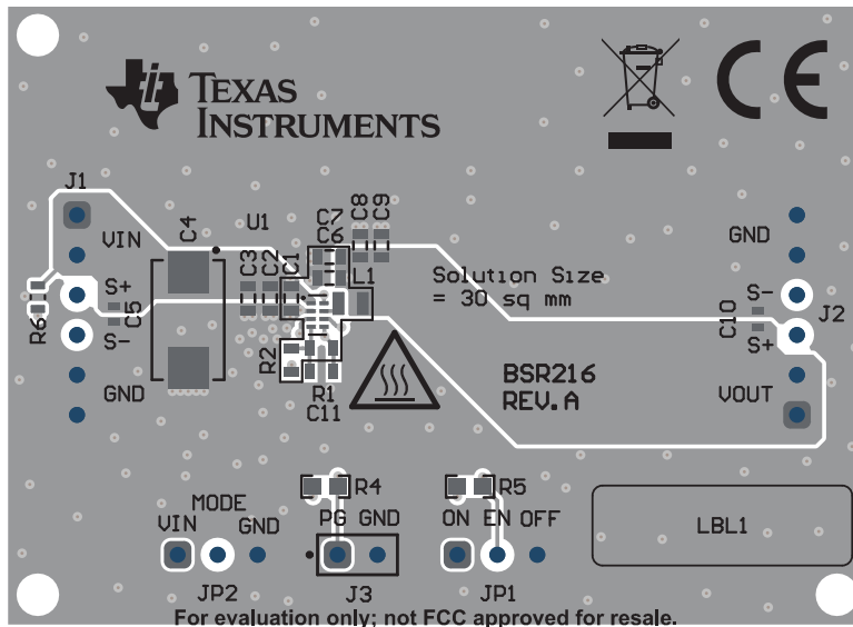
Figure 5-1. Top Assembly
