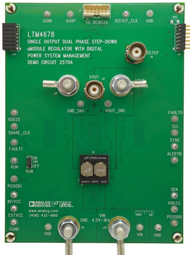
Figure 1. Single-Output 50A LTM4678/DC2570A Demo Circuit
