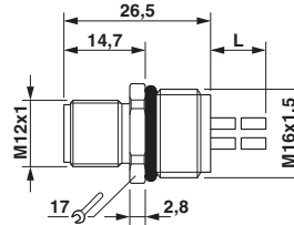
Dimensioned drawing
