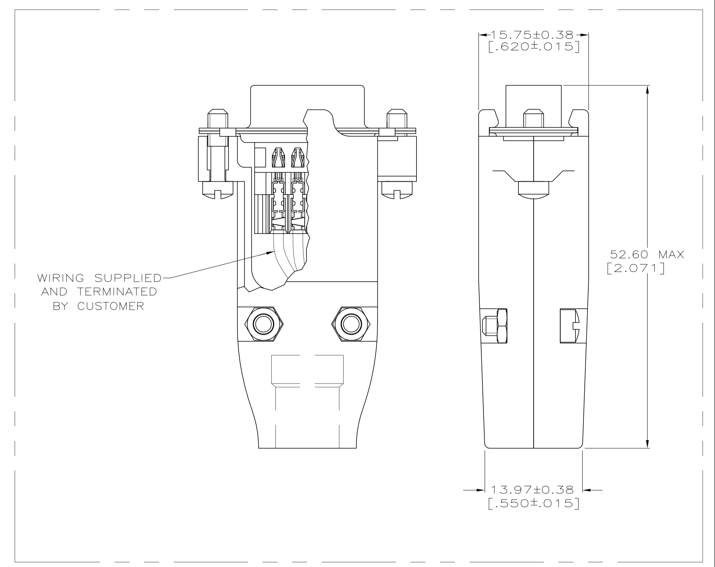
ASSEMBLED VIEW
