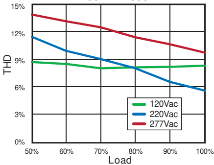
Total Harmonic Distortion 700mA model
