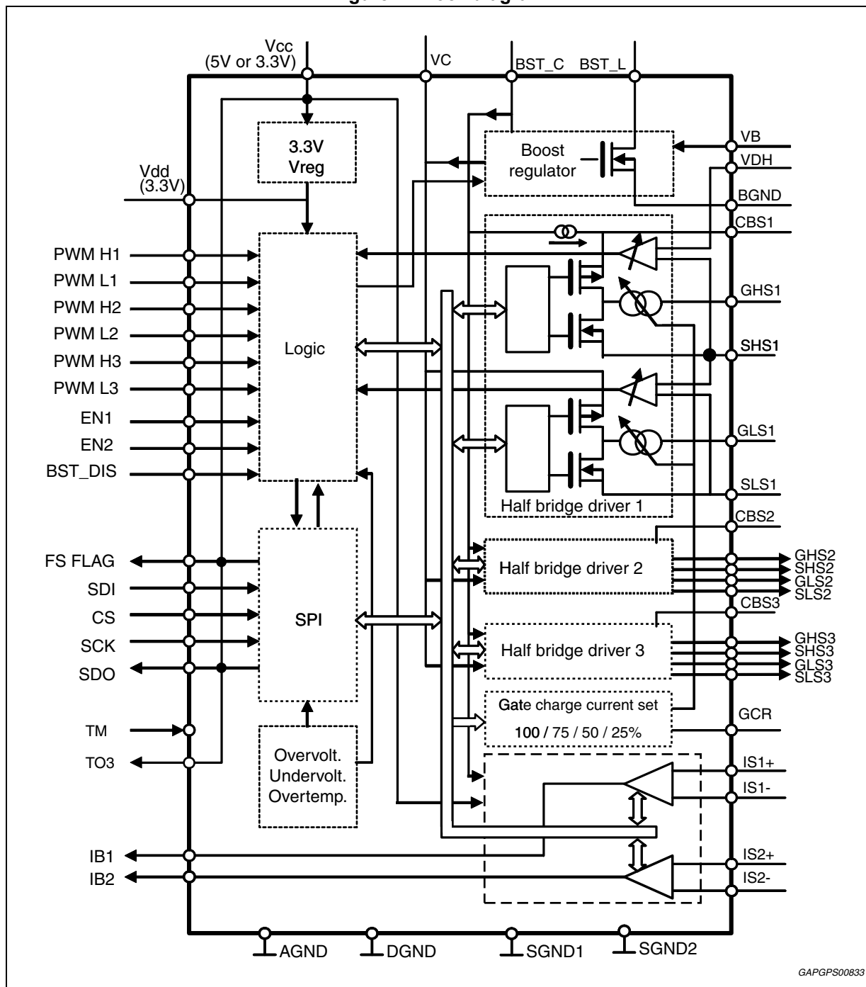
Figure 1. Block diagram
