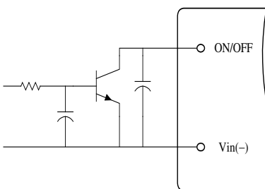
Figure 11. Open Collector Enable Circuit
