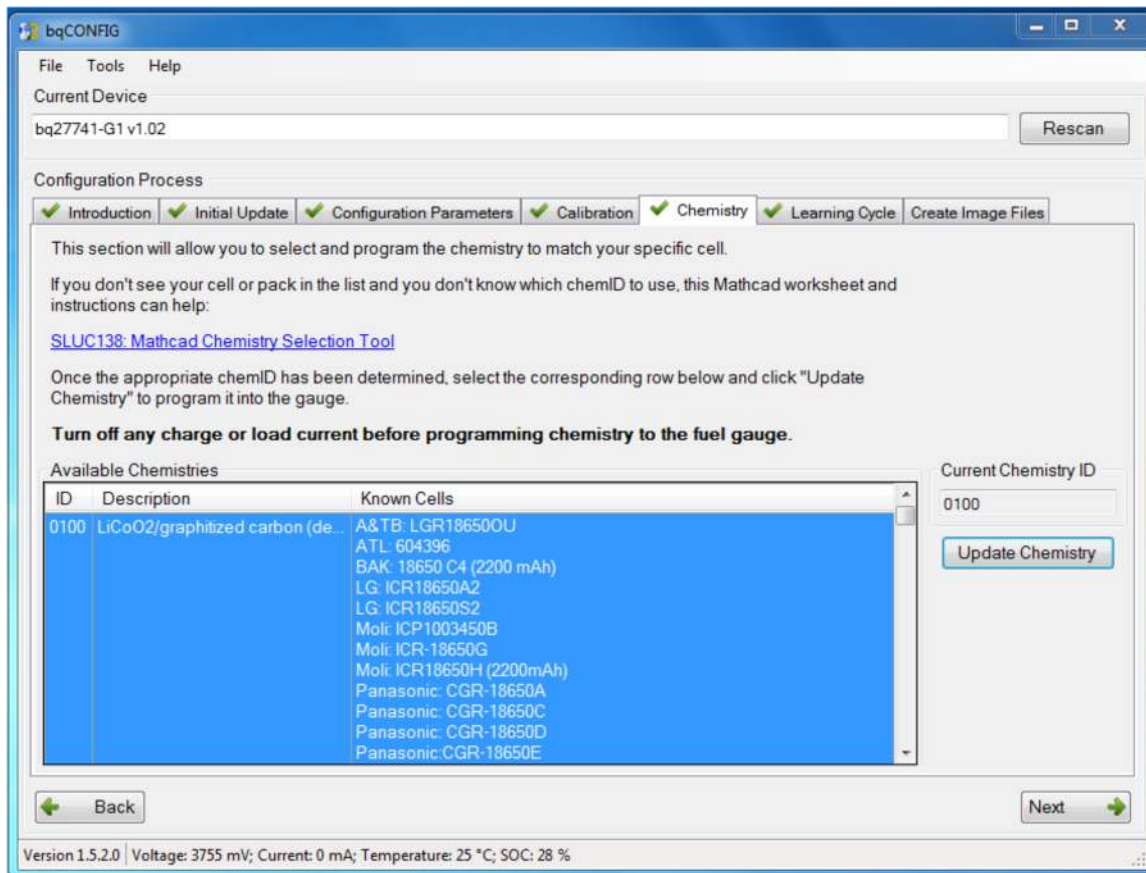
Figure 14. Chemistry Screen
