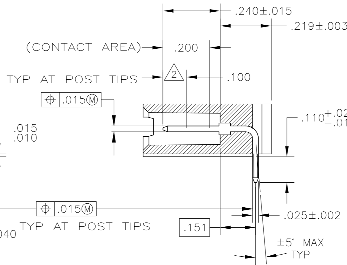
SECTION X-X
