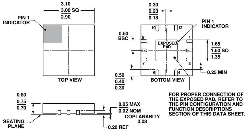
Figure 18. 12-Lead Lead Frame Chip Scale Package [LFCSP] 3 mm x 3 mm Body and 0.75 mm Package Height (CP-12-5) Dimensions shown in millimeters
