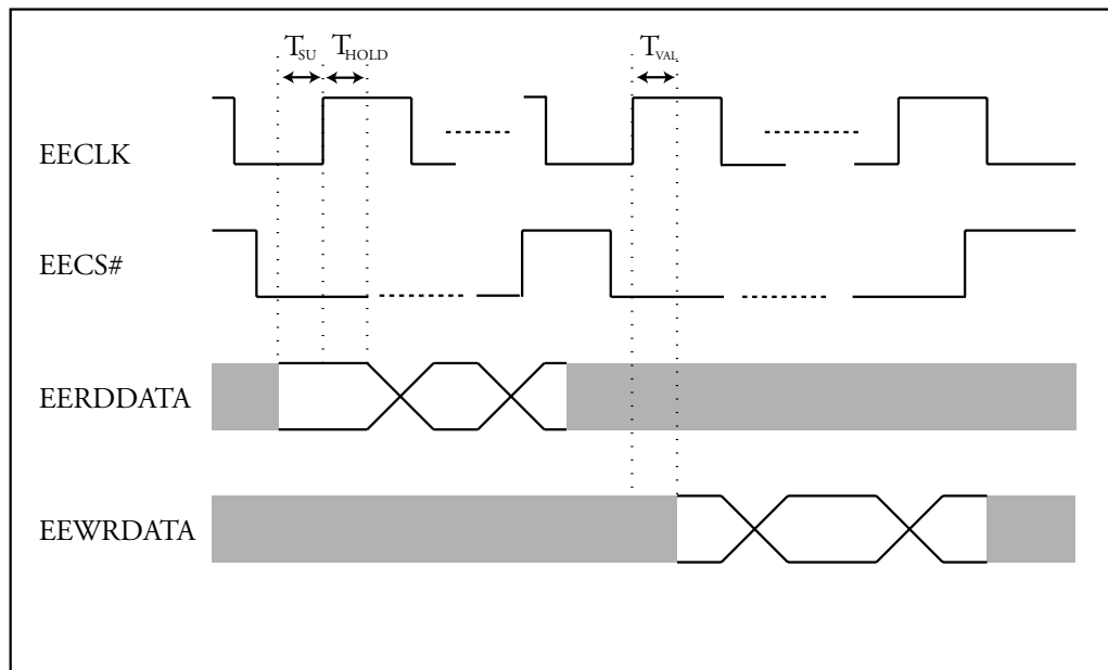
Figure 19-6. Serial EEPROM Timing Diagram
