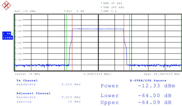
Figure 21. DAC3154 ACPR LTE 10-MHz FDD E-TM 1.1
