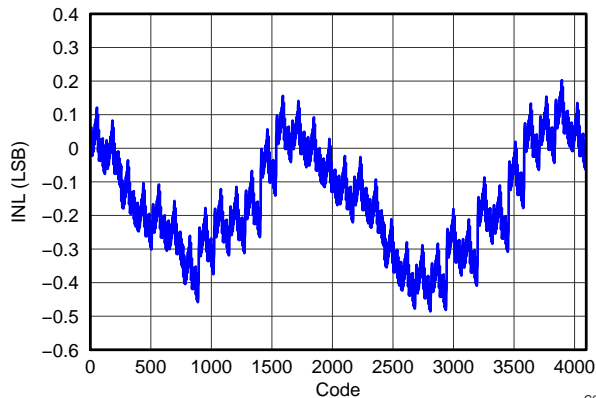
Figure 24. DAC3164 Integral Nonlinearity
