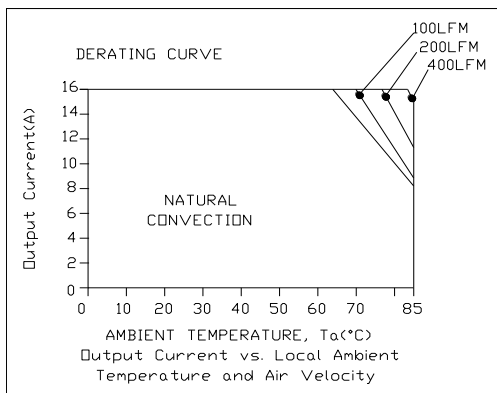
xRSB-40UV5x, Vin=18V
