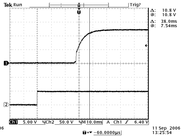
Startup time
