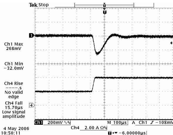
Vout=5.0 V 25% to 50% Load Transients
