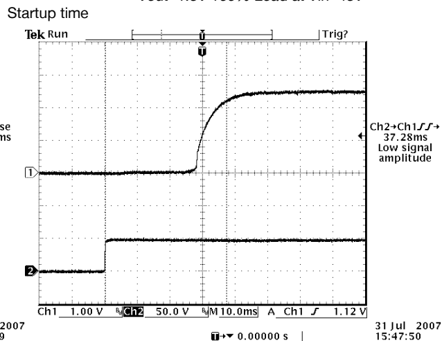
Vout=1.8V 100% Load at Vin=48V
