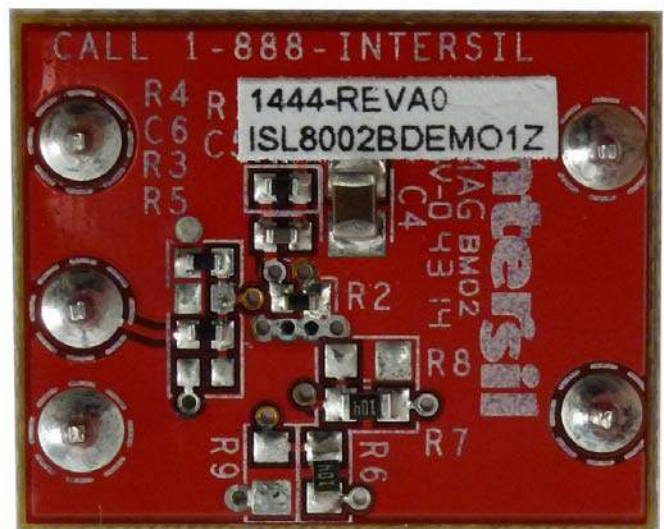
FIGURE 2. ISL8002BDEMO1Z BOTTOM SIDE
