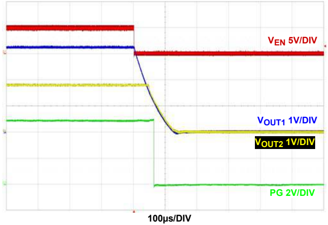
FIGURE 12. COINCIDENTAL VOLTAGE TRACKING SHUTDOWN AT FULL LOAD, V_{IN} = 5V , MODE = PWM, T_A = +25^\circ C
