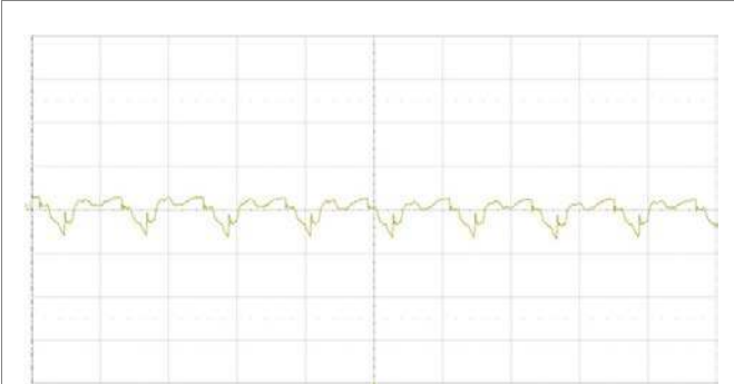
Output voltage ripple at: T_{P1} = +25^{\circ}\text{C} , V_i = 24\text{ V} , I_o = 15\text{ A} resistive load. Trace: output voltage (20 mV/div.). Time scale: (2 μs/div.). 20 MHz bandwidth.
