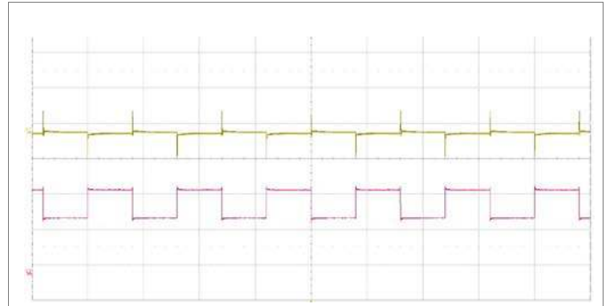
Output voltage response to load current step-change (1.7-2.55-1.7 A) at: T_{P1} = +25^{\circ}\text{C} , V_I = 24\text{ V} . Top trace: output voltage (500 mV/div.). Bottom trace: load current (1 A/div.). Time scale: (10 ms/div.).
