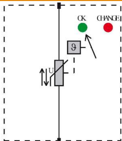
Schematic circuit diagram
