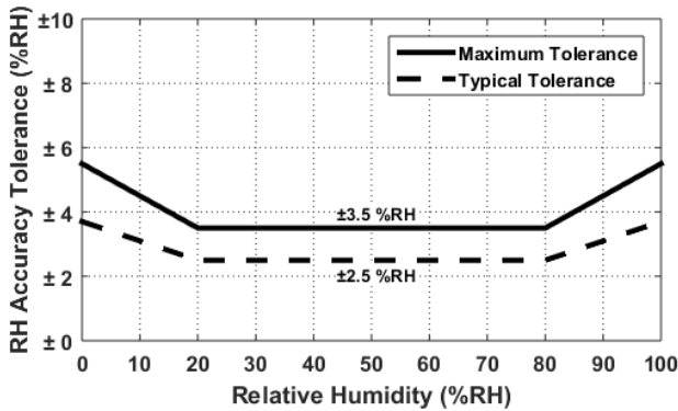
Figure 4. HS3103-ML1 RH Accuracy Tolerance at 25°C
