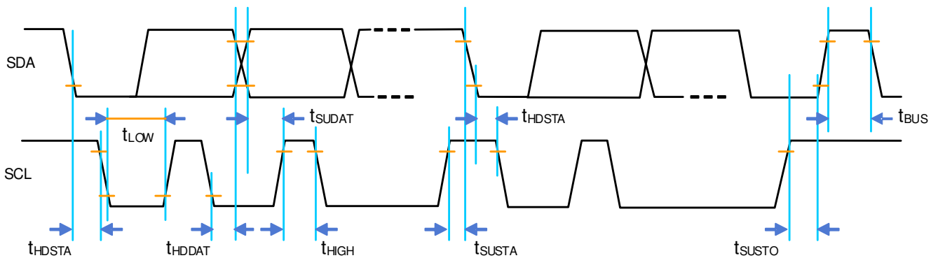
Figure 8. Timing Diagram
