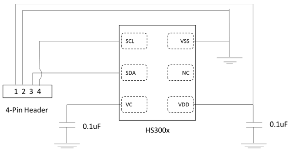
Figure 14. HS310x-ML1 Application Circuit
