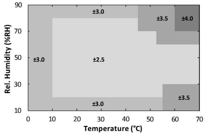
Figure 5. HS3103-ML1 RH Accuracy over Temperature
