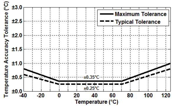
Figure 7. HS3103-ML1 Temperature Sensor Accuracy Tolerance
