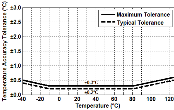
Figure 6. HS3101-ML1 Temperature Sensor Accuracy Tolerance
