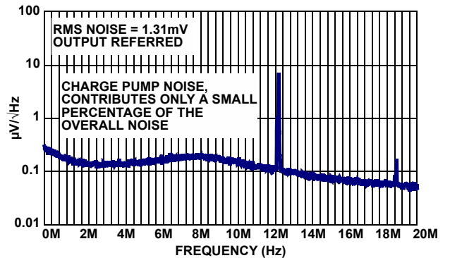
FIGURE 24. NOISE SPECTRUM
