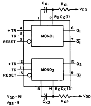
Dual Monostable Multivibrator
