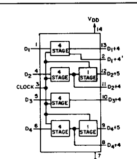
18-Stage Static Shift Register
