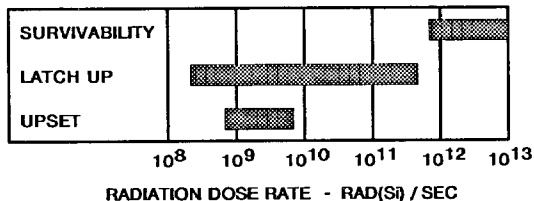
EFFECTS OF TRANSIENT RADIATION ( 10^6 RADS (Si) ON CD4000-SERIES INTEGRATED CIRCUITS (ALUMINUM GATE CMOS ON BULK SILICON)
