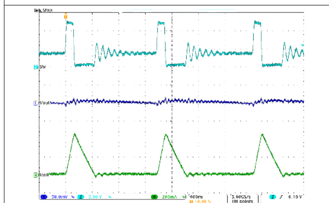
Iout = 66 mA
