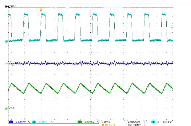
Iout = 1 A
