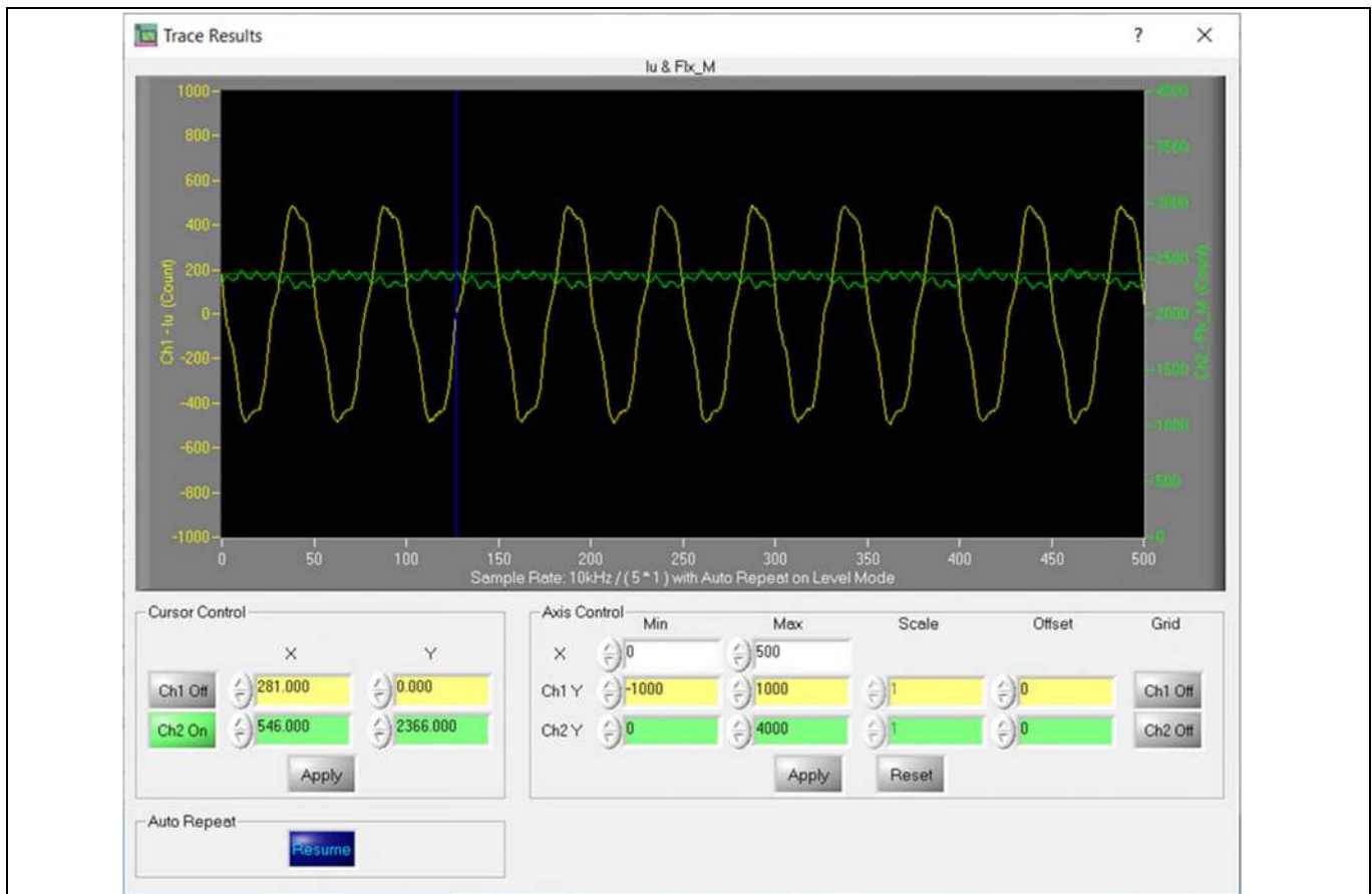
Figure 11 Trace waveform for I_u & Flx -M at 50% speed
