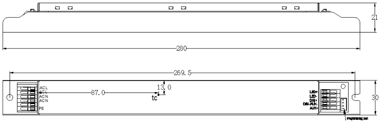
Figure 11: Mechanical Drawing
