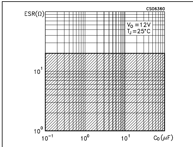
Figure 25. Stability
