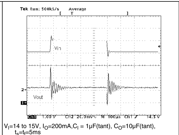
Figure 26. Line transient
