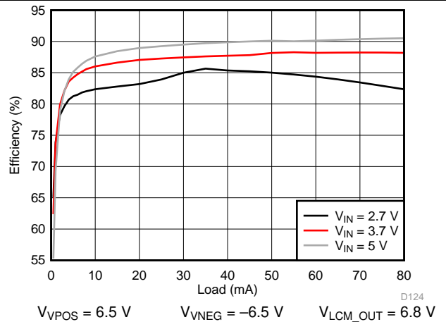
Figure 210. VPOS/VNEG Efficiency
