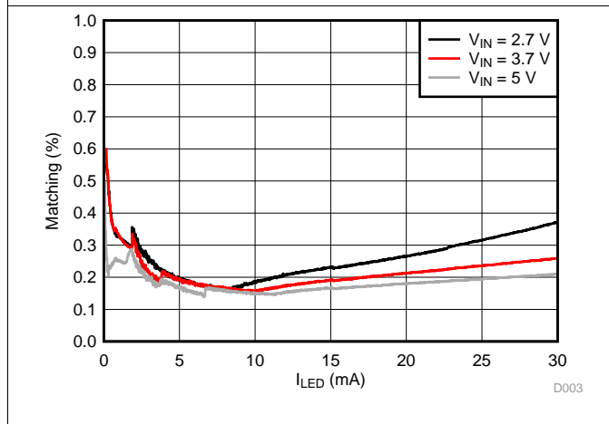
Figure 4. Backlight LED Current Matching
