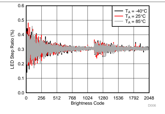
Figure 7. Backlight LED Current-Step Ratio
