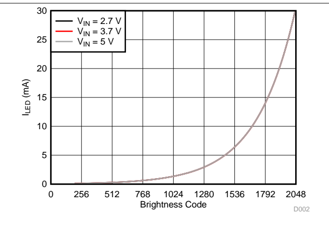
Figure 3. Backlight LED Current, Exponential Control
