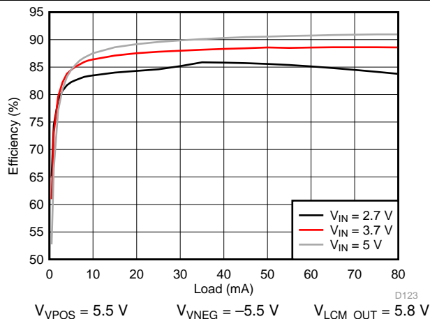
Figure 209. VPOS/VNEG Efficiency
