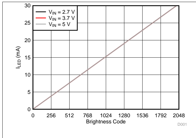
Figure 2. Backlight LED Current, Linear Control
