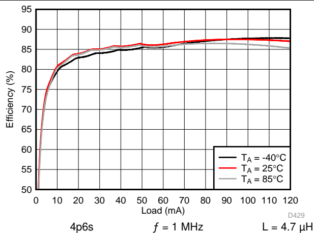
Figure 177. Backlight Boost Efficiency
