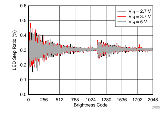
Figure 6. Backlight LED Current-Step Ratio
