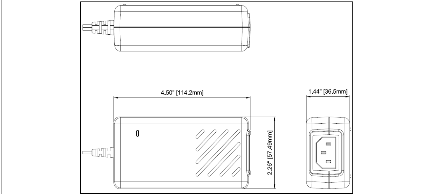
FWE050-Class I-DWG
