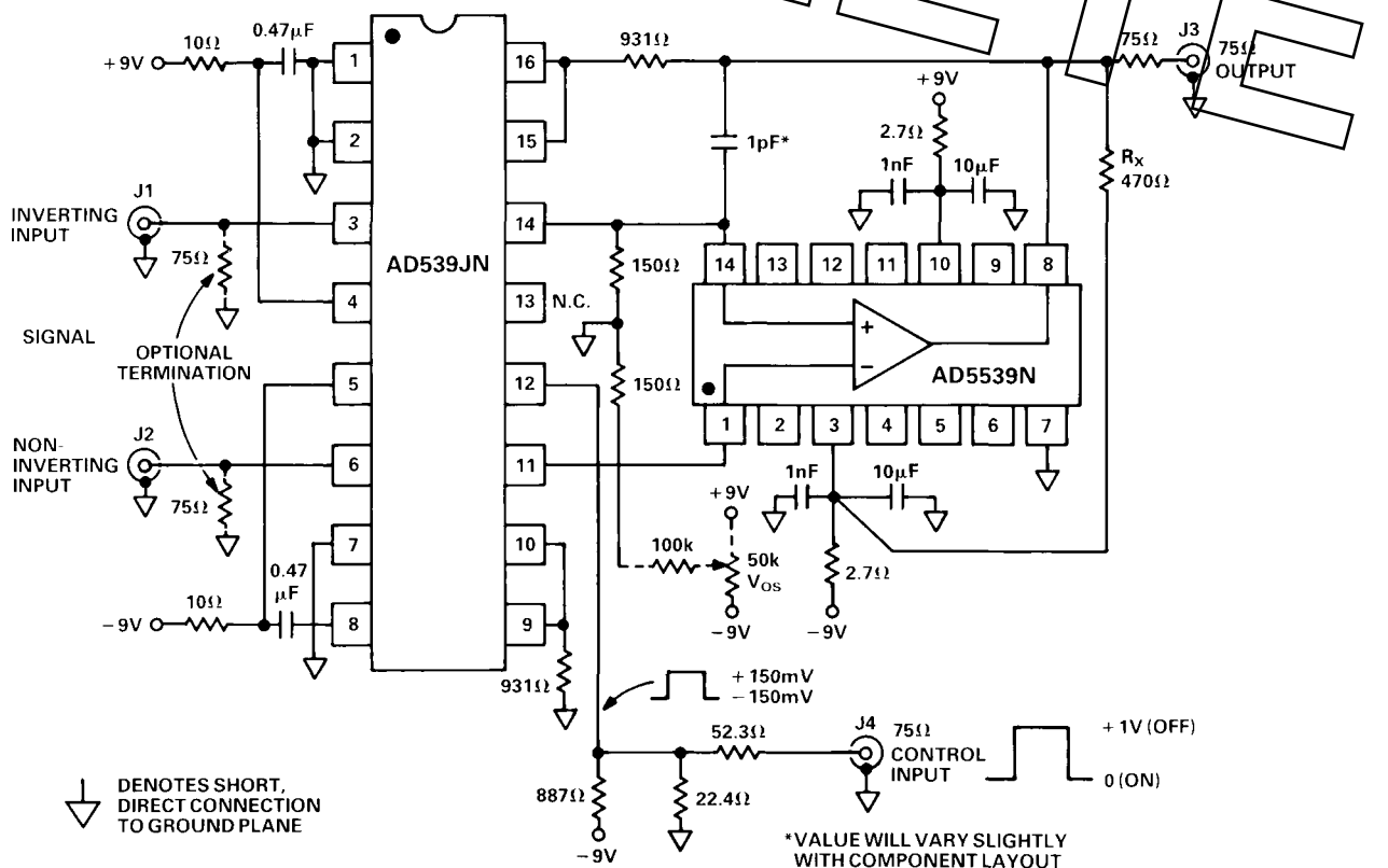
Figure 47. An Analog Multiplier Video Switch
