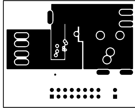
Figure 31. Layer 2 (GND)
