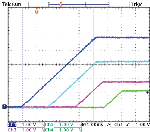
Figure 11 Sequential Start-up
