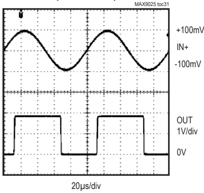
10kHz FREQUENCY RESPONSE ( V_{CC} = 1.8V )
