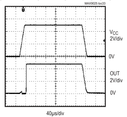
POWER-UP/POWER-DOWN RESPONSE
