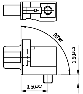
Detail of plastic pin
