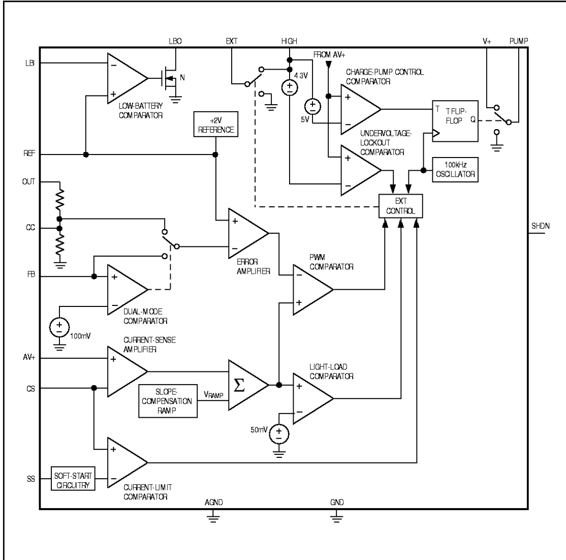
Figure 2. Block Diagram
