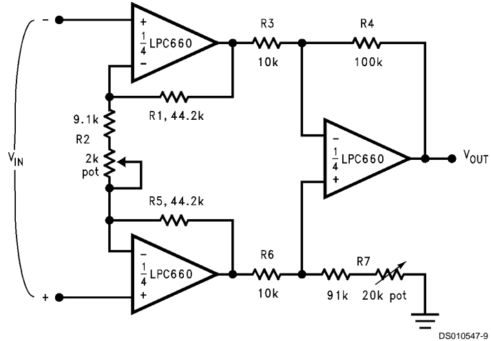
Instrumentation Amplifier
