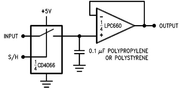
Low-Leakage Sample-and-Hold
