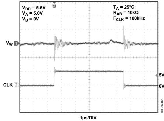
Figure 24. Digital Feedthrough
