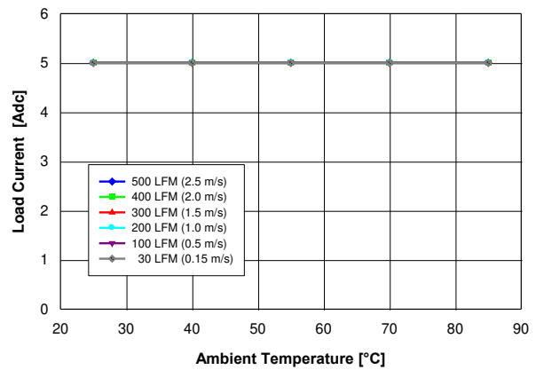
Fig. 3.3V.2: Available load current vs. ambient temperature and airflow rates for V_{out} = 3.3\ \text{V} converter mounted horizontally with V_{in} = 5\ \text{V} , air flowing from pin 5 to pin 1, and maximum MOSFET temperature \leq 120^\circ\text{C} .
