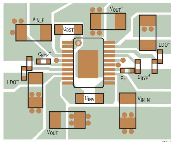
Figure 6. Recommended Layout
