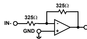
FIGURE 22. A_V = -1
