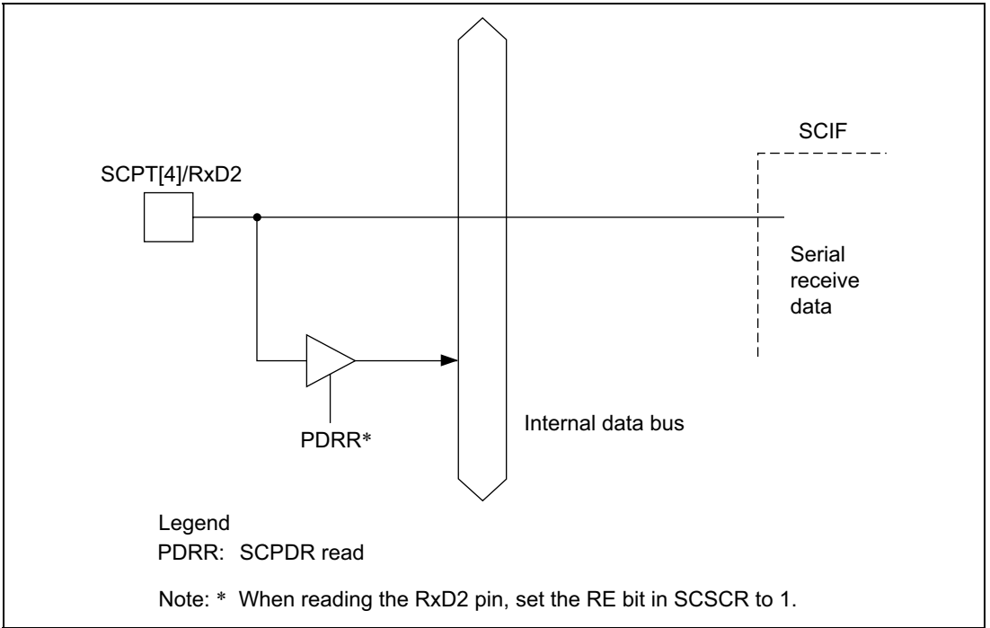
Figure 16.4 SCPT[4]/RxD2 Pin
