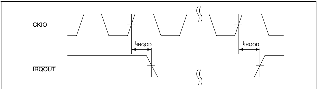
Figure 23.13 \overline{\text{IRQOUT}} Timing
