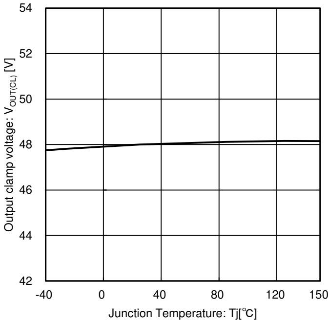
Figure 7. Output clamp voltage vs. Junction Temperature
