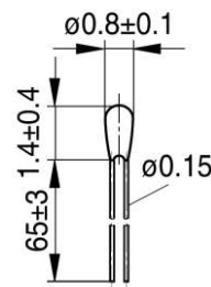
Figure 2. Side View of ATH10KR8B
