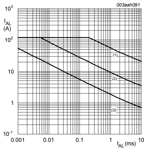
Fig. 4. Single pulse avalanche rating; avalanche current as a function of avalanche time
