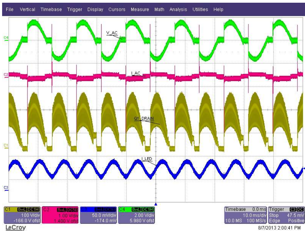
Figure 18. Leading-edge Dimmer Mode, Steady-state, 120VAC
