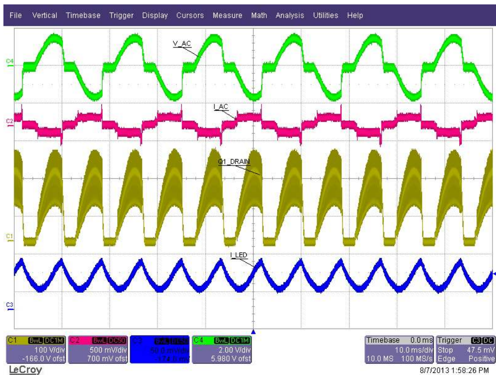
Figure 19. Trailing-edge Dimmer Mode, Steady-state, 120VAC
