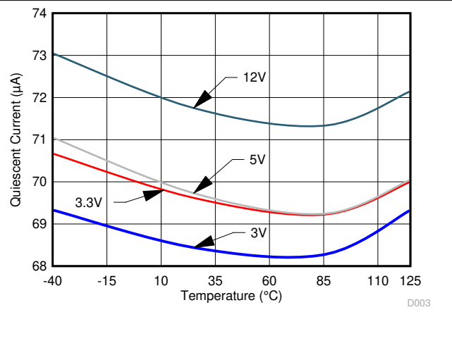
Figure 7-2. V_{IN} vs I_Q over Temperature
