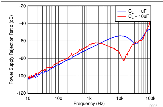
Figure 7-5. Power-Supply Rejection Ratio vs Frequency
