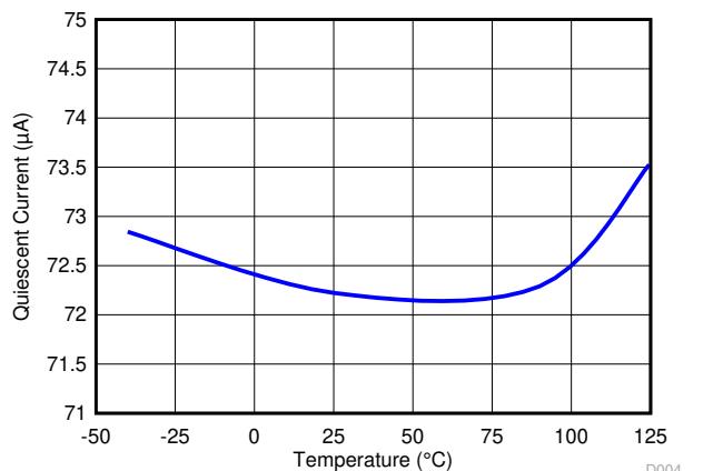
Figure 7-4. Quiescent Current vs Temperature
