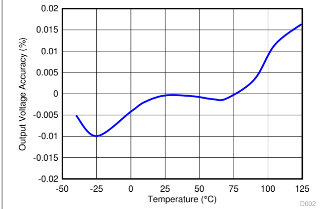
Figure 7-3. Output Voltage Accuracy vs Temperature
