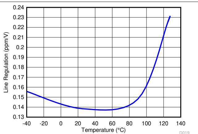
Figure 7-6. Line Regulation
