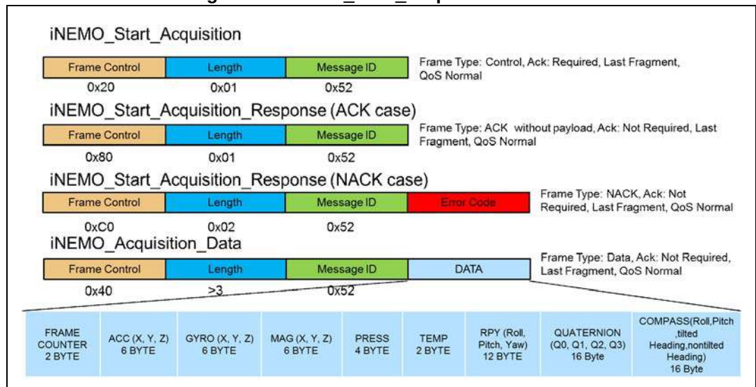
Figure 31. iNEMO_Start_Acquisition frames
