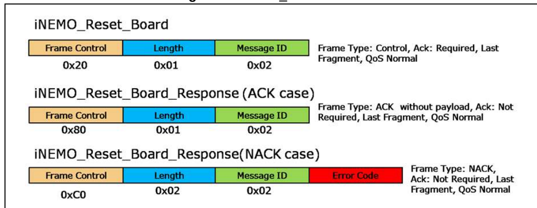
Figure 9. iNEMO_Reset frames
