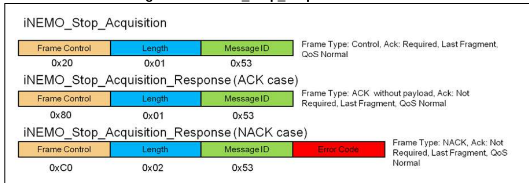
Figure 32. iNEMO_Stop_Acquisition frames
