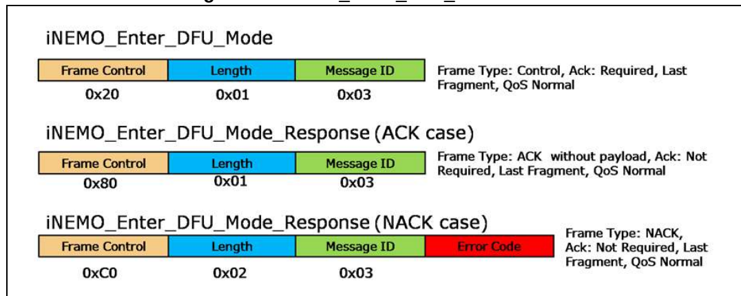
Figure 10. iNEMO_Enter_DFU_Mode frames
