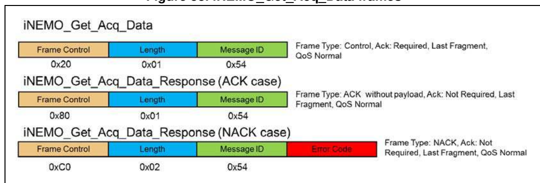
Figure 33. iNEMO_Get_Acq_Data frames
