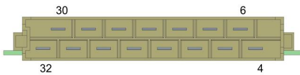
CONNECTOR DIN41612H15 - 12A / Terminal
