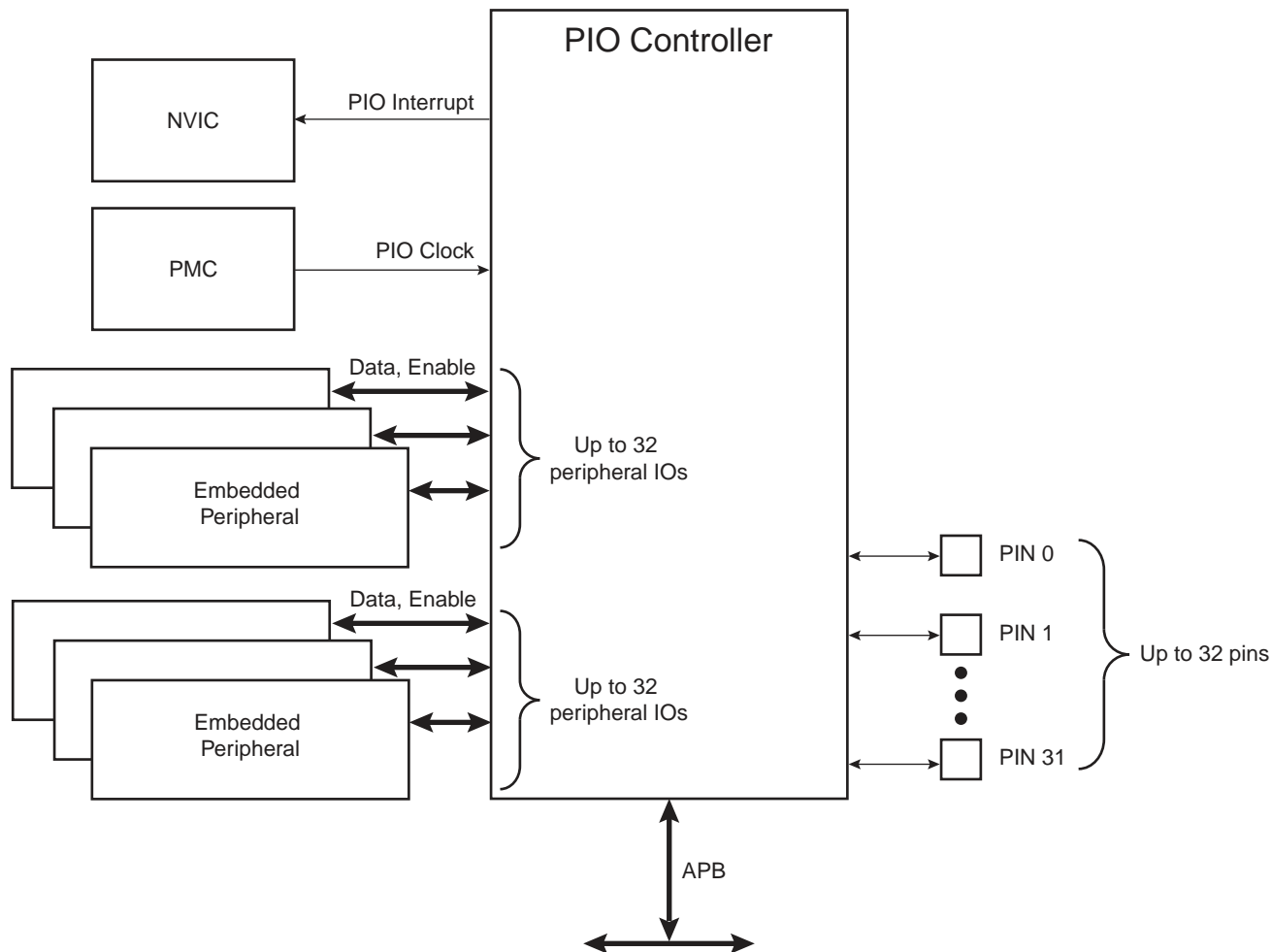
Figure 29-1. Block Diagram
