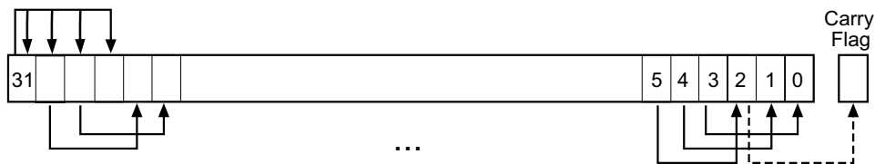
Figure 12-4. ASR #3
