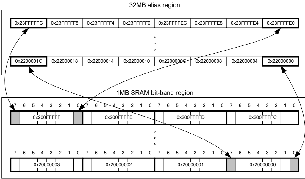
Figure 12-2. Bit-band mapping
