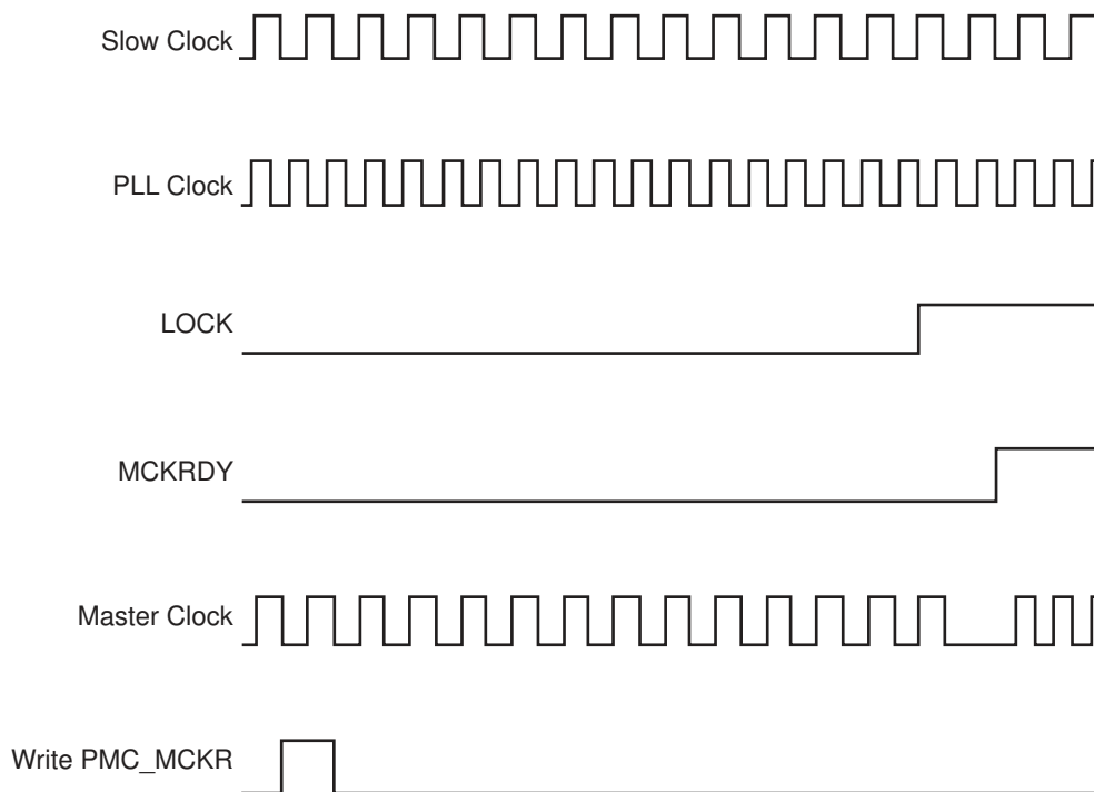
Figure 27-4. Switch Master Clock from Slow Clock to PLL Clock
